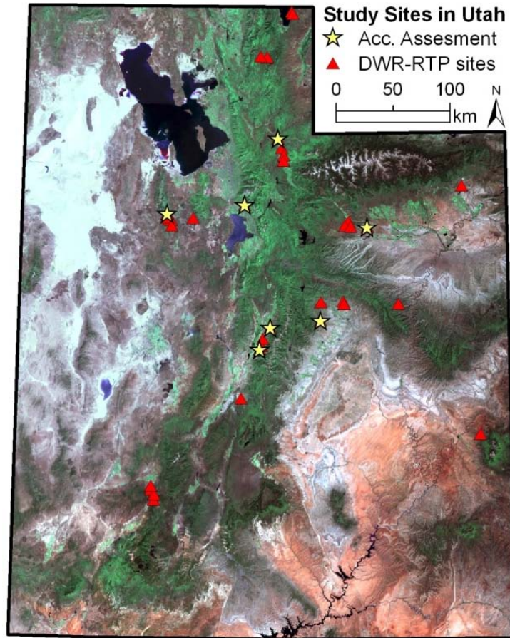
Fig. 1. Landsat TM imagery (Utah State University, 2001) of the state of Utah, overlaid by Utah Division of Wildlife Resources Range Trend Project (DWR-RTP) locations analyzed through feature extraction techniques, and those DWR-RTP sites for which ground reference measurements were also performed for in-situ accuracy assessments. Imagery obtained from Intermountain Region Digital Image Archive Center, Utah State University.
